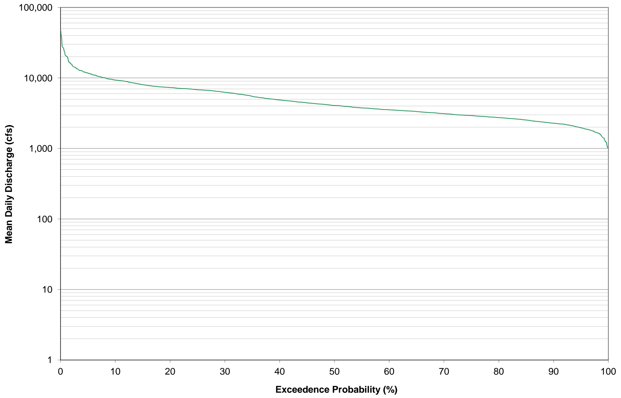
Platte River at Louisville USGS Gage 06805500 Monthly Flow Duration Curve - October Period of Record: CY 1950 - CY 2010
