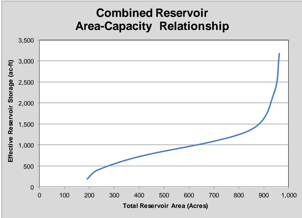
Graph B-2. Reservoir Area Capacity Curve
