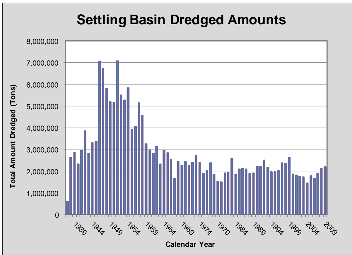
Graph B-1. Loup Power District Settling Basin Dredging History
